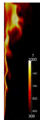
FIGURE 2 – Wall flame simulation
